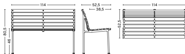
TRAVERSE DINING BENCH Width 114 cm Depth 52,5 cm Height 80,5 cm Seat height 46 cm Seat depth 38,5 cm
