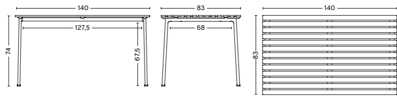
TRAVERSE TABLE Length 140 cm Width 83 cm Height 74 cm
